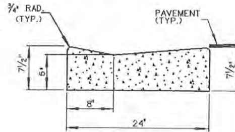
PALM BEACH MOUNTABLE GUTTER
