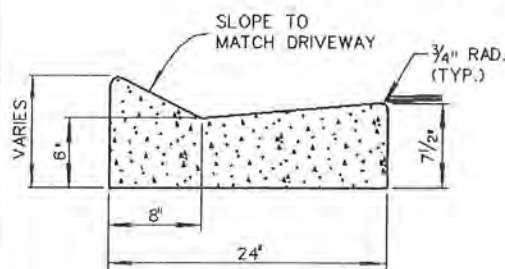
DRIVEWAY CURB
