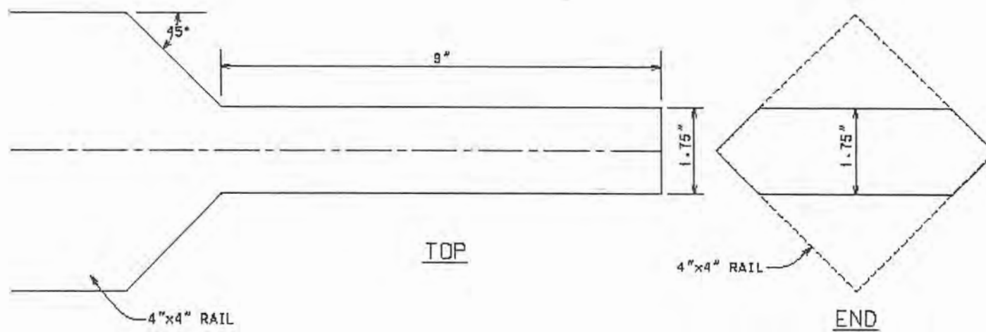
RAIL END DETAIL SCALE: 1" = 2"
