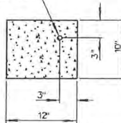
FLUSH HEADER CURB
